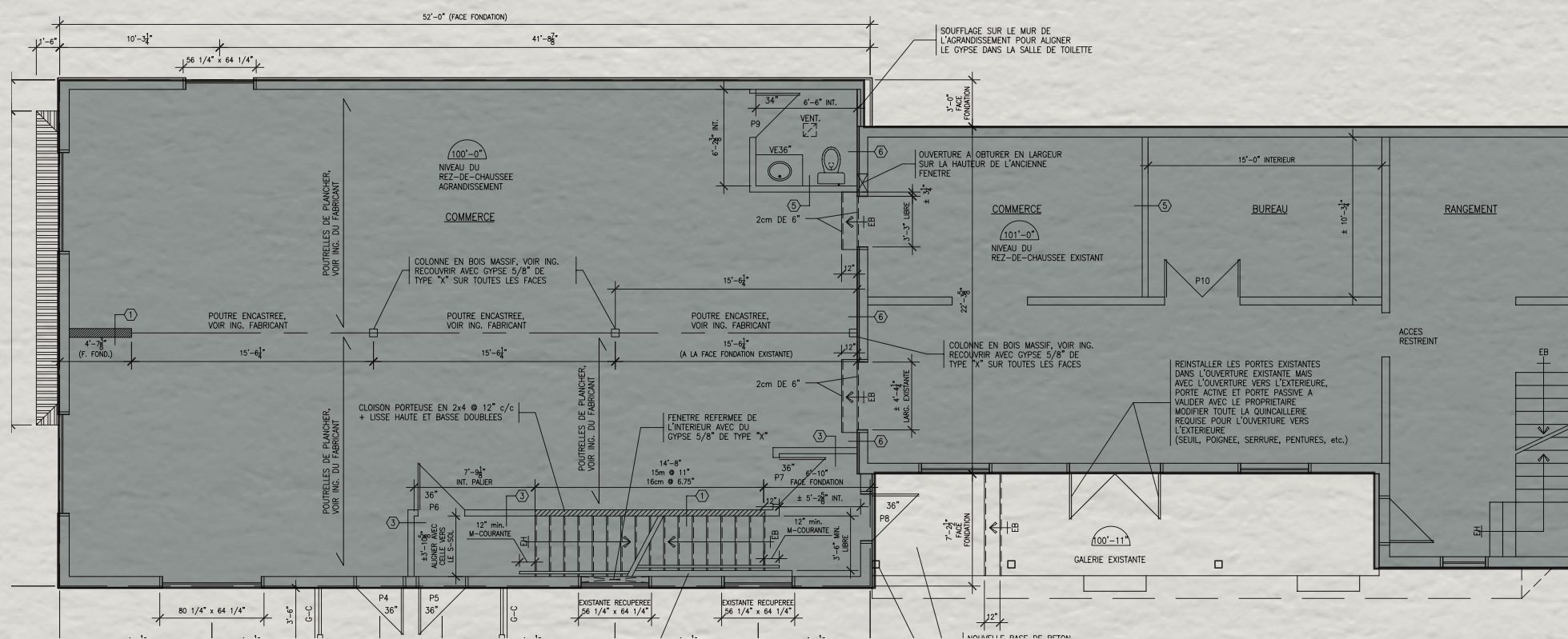
Ground Floor
